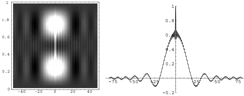
Figure 2. Left: the spectral density \sigma_G(\omega, \underline{x}, \underline{y}) for \underline{x} = (x, 0, 0) , \underline{y} = (x, y, 0) as a function of x \in [0, a] and y \in [-50a, 50a] . Right: normalized spectral density \sigma_G(\omega, \underline{x}, \underline{y})/\sigma_G(\omega, \underline{x}, \underline{x}) for y \in [-50a, 50a] at x = 0.75a (symmetrically including 1000 terms of the n -sums). All distances are in \mu\text{m} , the frequency is \omega = 2\pi c/a and the plate separation a = 1 \mu\text{m} .
