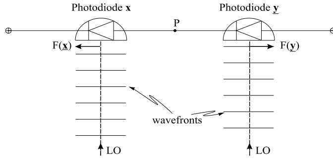
Figure 1. BHD with a LO. Note, that the setup is arranged in such a way, that the electric field of the LO at \underline{x} has a reversed direction w.r.t. that at \underline{y} .
