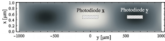
Figure 3. Experimental setup drawn on the plot of the F_y(\underline{x}) , the y -component of the electric field of \text{TE}_1 mode of the Casimir cavity. The mode, serving as the LO, propagates in the z -direction perpendicular to the plot.
