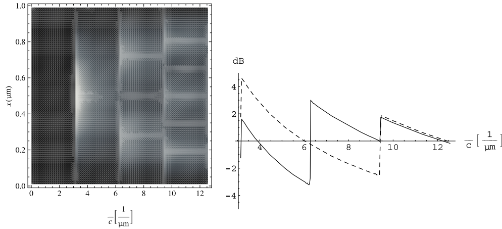
Figure 4. Left: Casimir spectral density normalized by vacuum spectral density, [\sigma_{yy}(\omega, \underline{x}, \underline{x}) - \sigma_{yy}^{\Omega}(\omega, \underline{x}, \underline{x})]/\sigma_{yy}^{\Omega}(\omega, \underline{x}, \underline{x}) as a function of the distance x \in [0, a] . Negative (sub-vacuum) values are black. Right: suppression of vacuum fluctuations (see the text) in dB for x = 0.25a (solid) and x = 0.5a (dashed). Frequency range is \omega \in [0, 4\pi c/a] ; a = 1 \mu\text{m} is assumed.
